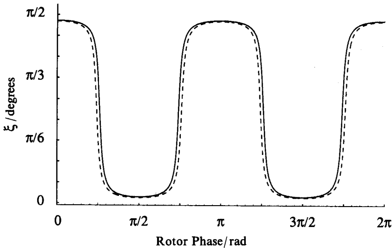
Figure 1. Plots of \xi_1 (— — —) and \xi_2 (————) as functions of rotor phase for a crystallite spinning about the magic angle ( 54.74^\circ ) with PAS oriented perpendicular to the rotor, \epsilon^2 qQ/h = 11.0 MHz and \eta = 0.0 .
