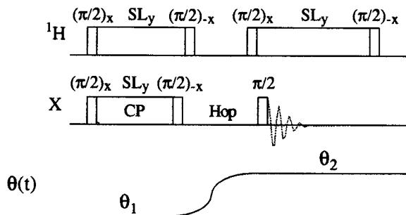
Figure 7. One-dimensional ZPVAS pulse sequence. The axis angle with respect to time is shown below the sequence. SL refers to spin lock. Subscripts refer to the phases of pulses.
