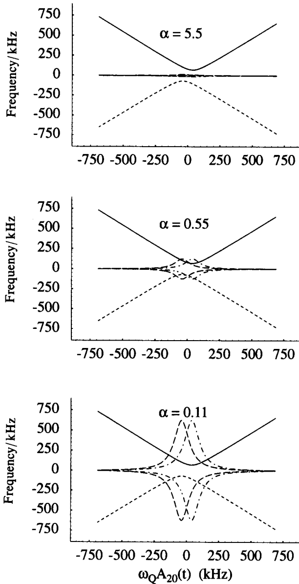
Figure 2. Plot of diagonal and off-diagonal coefficients \omega^{1-3} (—), \omega^{2-4} (- - -), d(2\xi_1)/dt (- · -) and d(2\xi_2)/dt (— — —) of the time-dependent frame Hamiltonian in equations (13) and (20), as functions of \omega_Q A_{20}^Q(t) . The off-diagonal coefficients have the form of Lorentzian impulse functions as follows:
